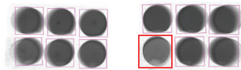
Figure 16: Twin lane inspection of six-pack yoghurts with one low fill
